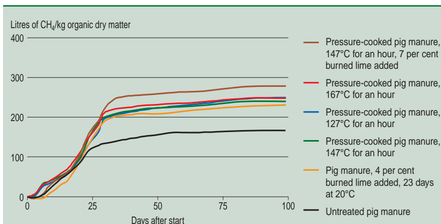
Figure 3. Results of laboratory testing of digestion of untreated manure fibres and pressure-cooked material with and without addition of burned lime.
